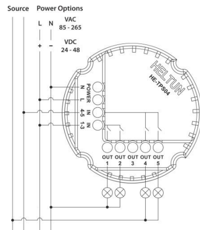
Connection Diagram 4
