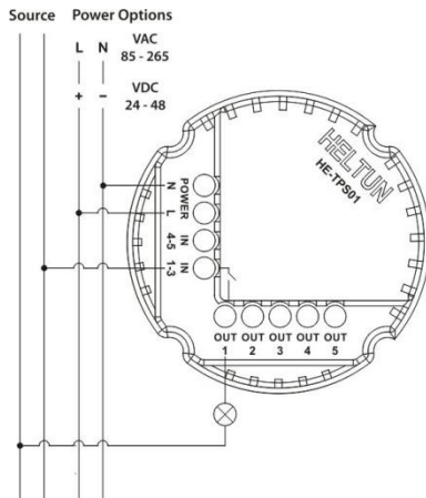
Connection Diagram 1
