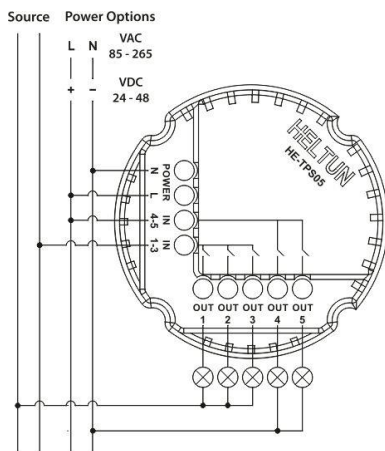
Connection Diagram 3
