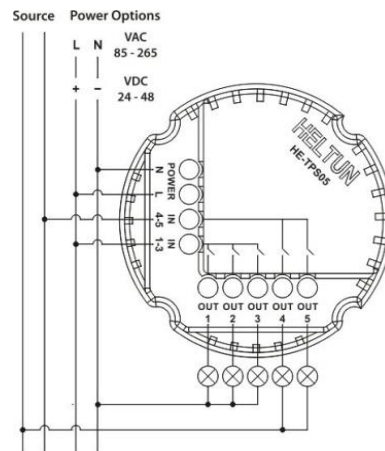
Connection Diagram 4
